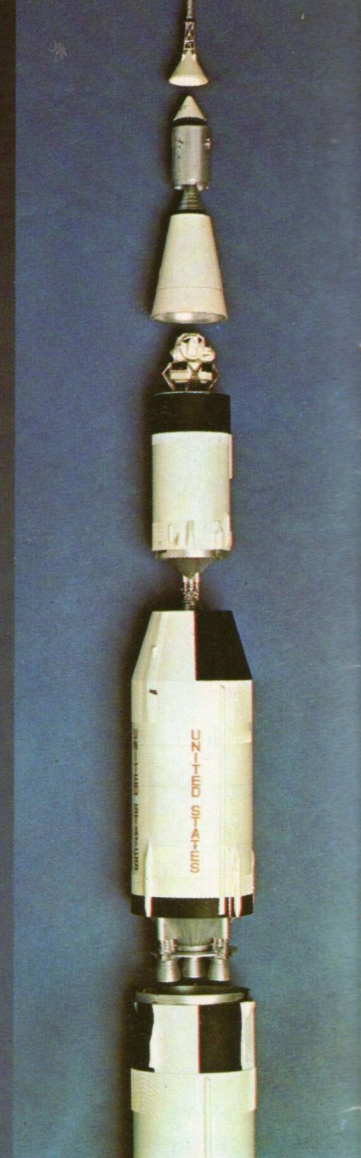
Exploded picture of the Saturn V rocket.
