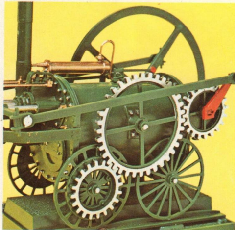
Steam Locomotive: close-up of driving wheels.
