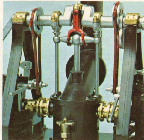
Paddle Engine: crankshaft and piston detail.
